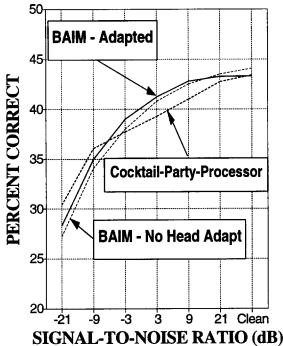
Figure 2. Cocktail-Party-Processor vs BAIM
