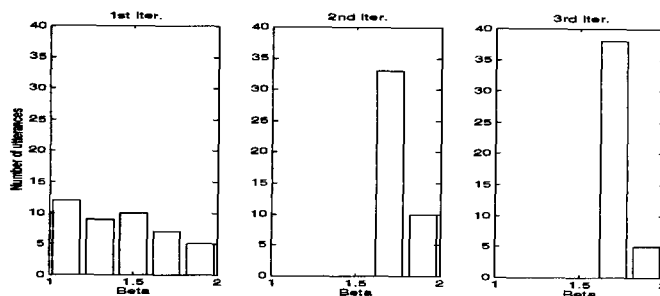
Figure 3. Warping selected for utterances of a female talker through iteration 1 to 3.
