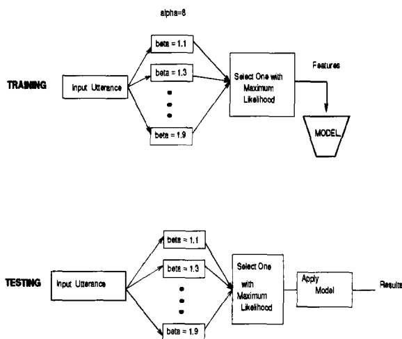
Figure 2. The algorithm for training and testing.
