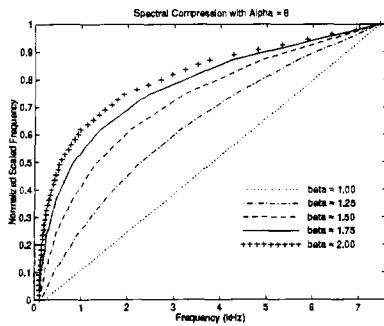
Figure 1. Spectral warping with \alpha = 8.0 .
