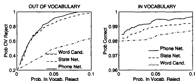
Figure 1: Performance comparison using different representations for the alternate hypothesis model. a) ROC's for OOV word rejection vs. the INV rejection b) ROC's for INV word detection vs. the INV rejection.
