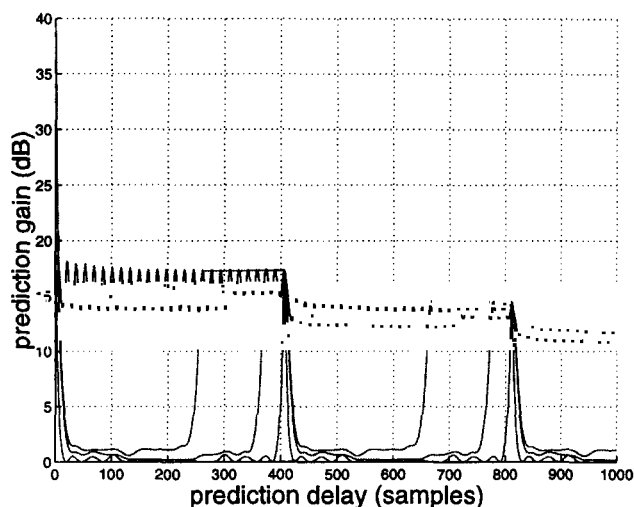
Figure 1. Linear prediction gain vs. prediction delay: Long-memory linear predictor (oscillating behavior); short-memory linear predictors, D = 1/33/144 (smooth curves with peaks at multiples of the pitch period).
