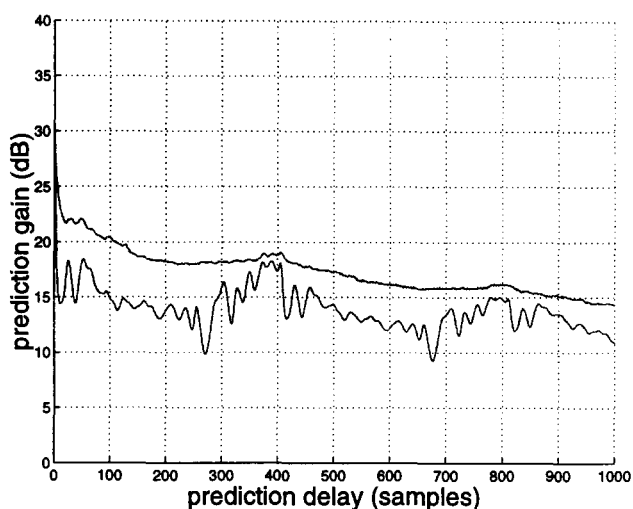
Figure 2. Nonlinear prediction gain vs. prediction delay: Upper bound obtained from the mutual information estimate (top); short-memory RBF-AR predictor, D = 3 (bottom).
