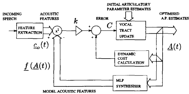
Figure 1: Using an MLP in an analysis-by-synthesis scheme with the inclusion of dynamic constraints.
