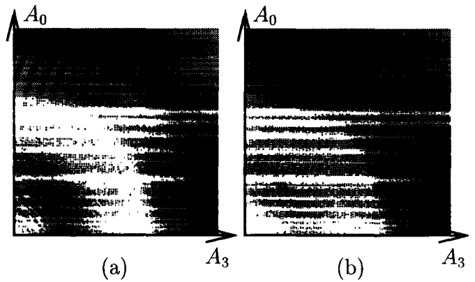
Figure 2: The acoustic cost function for an [r] spectrum with two articulatory parameters (a) without and (b) with distributed losses taken into account.
