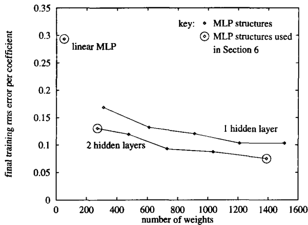
Figure 3: Final training error for different MLP topologies. MLPs with 10 to 30 units in each hidden layer are shown. The MLPs used in Section 6 are highlighted. For reference, the rms 'error' with respect to the mean of the training data is 0.38.
