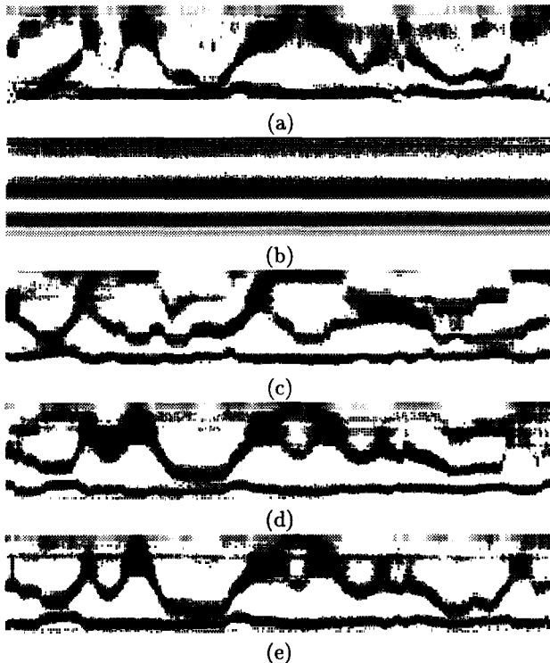
Figure 5: Linear MLP initialisation of MLP analysis-by-synthesis of utterance 'Why were you away a year ago Roy'. PLP-derived spectrograms are shown of (a) the original speech, and the spectral output of the vocal tract shapes of (b) the uniform tube initialisation, and after optimisation using (c) the linear MLP, (d) a 2 hidden-layer MLP with 10 hidden units in each layer, and finally (e) a 2 hidden-layer MLP with 30 hidden units in each layer.
