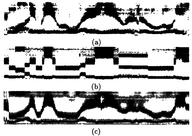
Figure 4: MLP analysis-by-synthesis for the utterance 'Why were you away a year Roy'. PLP-derived spectrograms are shown of (a) the original speech, (b) the spectral output of the vocal tract shapes used for initialisation from a very small articulatory codebook (81 entries), and (c) the spectral output of the optimised vocal tract shapes.
