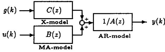
Fig.1 Glottal-ARMAX model
