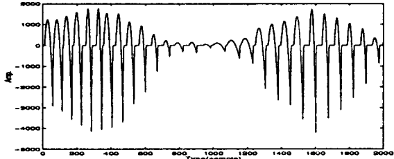
(10,6,6) ARMAX analysis
