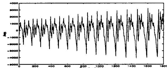
(a)Speech signal
