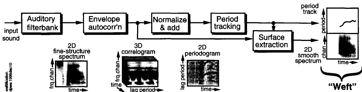
Figure 1: Calculation of a weft: The three-dimensional correlogram volume (the short-time envelope autocorrelation of filterbank output channels) is normalized and collapsed across channel to form a summary periodogram. Peaks in this result are extracted to produce the period-track portion of the weft. The correlogram volume is then sampled at that period to extract the smoothed spectrum of the weft for every channel at each time slice, taking care to factor-out interference from other energy in each channel.
