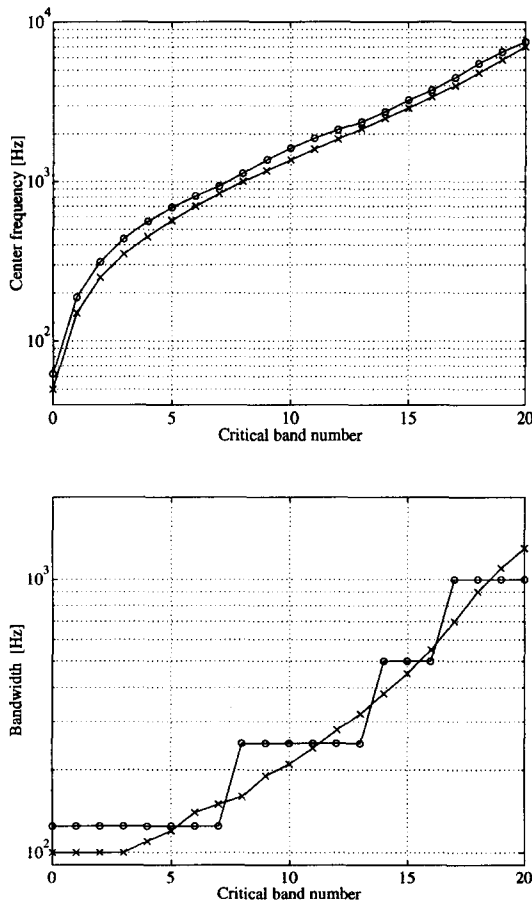
Figure 2. Approximation of the critical band decomposition. Top: center frequencies. Bottom: bandwidths. 'x' are reference values and 'o' are approximation values.
