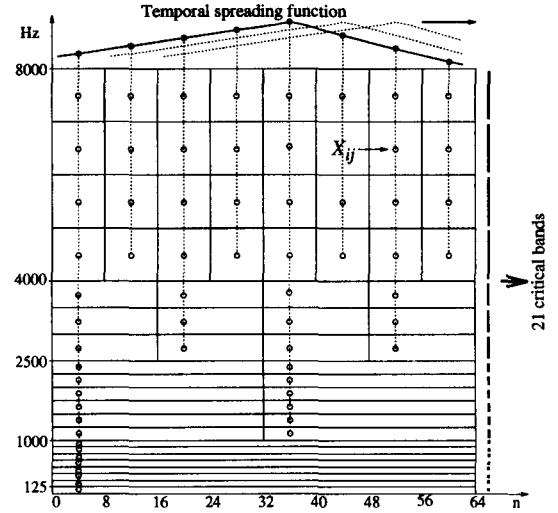
Figure 3. Time-frequency grid of the transform and calculation of temporal masking.
