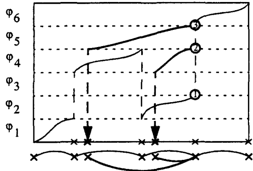
Fig 2: Lattice generation.
