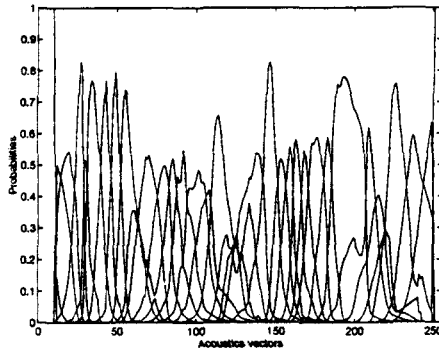
Fig 1: Phonemes transitions
