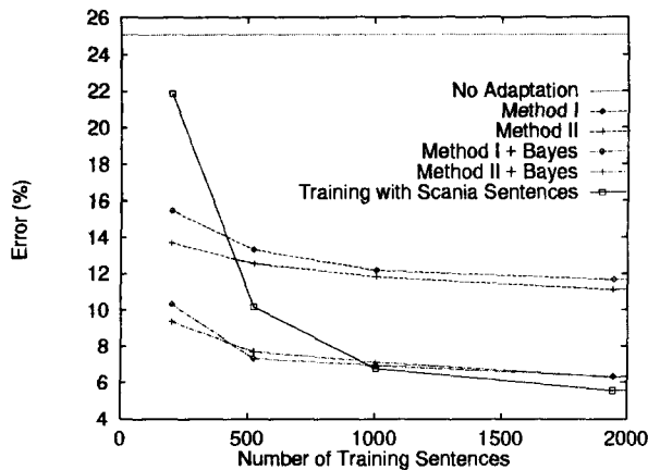
Figure 1. Dialect adaptation results for adaptation methods I, II, their combination with Bayes and standard ML training.
