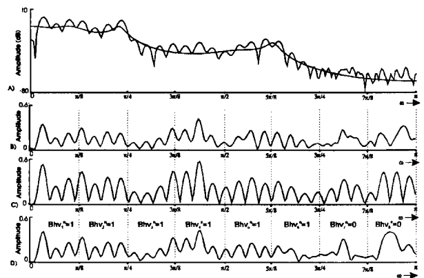
Figure 4. A) Short-term speech magnitude spectrum and LPC spectral envelope ( \log_{10} domain), and the short-term magnitude spectra of the corresponding: B) residual segment, C) excitation segment obtained using the binary excitation model, and D) excitation segment obtained using the mixed excitation model.
