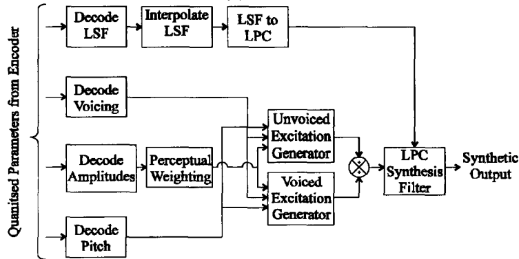
Figure 5: Decoder Schematic
