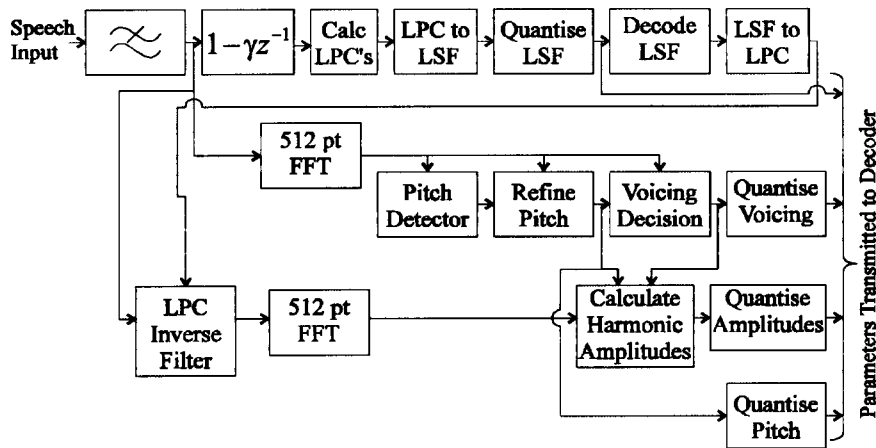
Figure 3: Encoder Schematic
