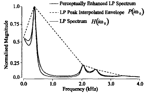
Figure 4: Effect of Perceptual Enhancing Process on LPC Spectrum
