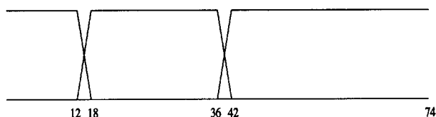
Figure 2. The frequency regions for quantising the extended prototype spectrum
