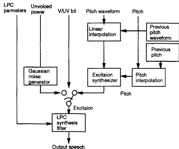
Figure 2. Block diagram of the decoder
