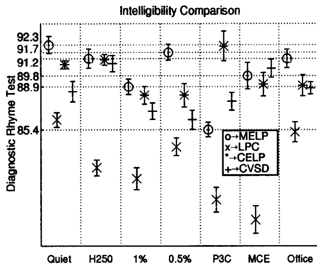
Figure 4: Intelligibility Comparison, Benign
