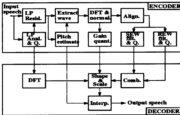
Figure 1. Basic waveform interpolation coder.
