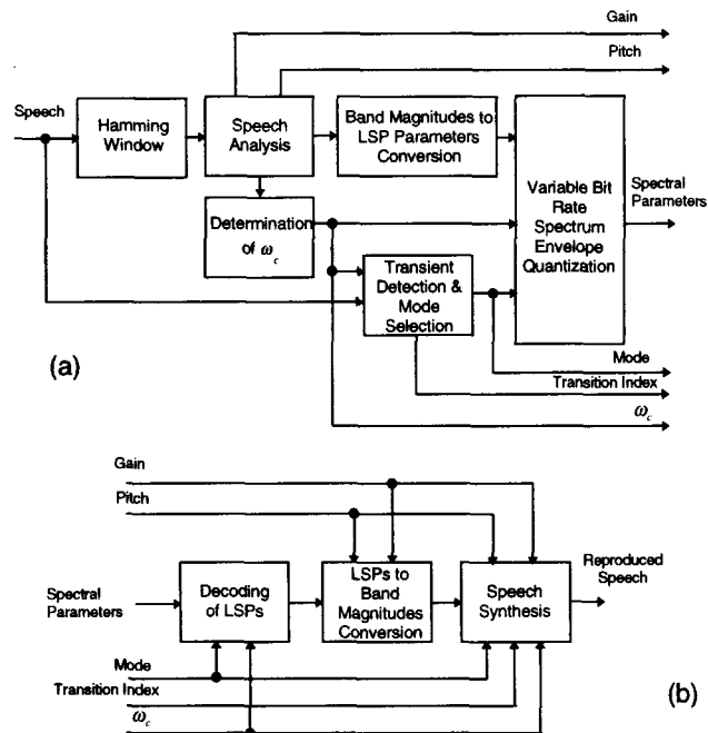
Figure 4 Block diagram of the variable bit rate MBELP coder: (a) encoder; (b) decoder.
