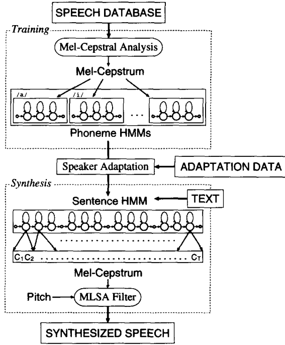
Figure 1: Block diagram of speech synthesis system.
