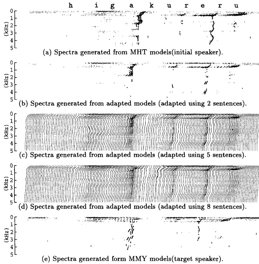
Figure 2: Generated spectra of the sentence “/h-i-g-a-k-u-r-e-r-u/”
