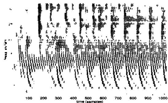
Figure 2: Sample Cochleagram
