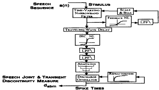
Figure 1: Carney Model Flow Diagram
