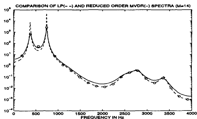
Figure 3. Comparison of normal LP spectrum (---), reduced order MVDR spectrum (—), and 186Hz Voiced Speech Harmonics (o), M=14
