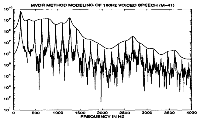
Figure 2. MVDR Spectrum of a 160Hz Voiced Speech Spectrum, M=41
