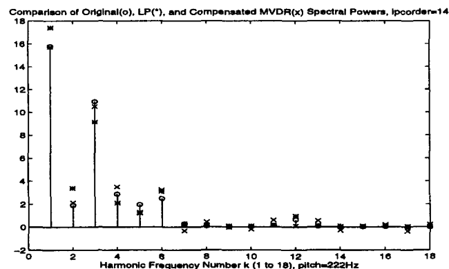
Figure 4. Comparison of original 222Hz voiced speech (o), LP (*), and compensated MVDR (x) spectral powers at the harmonics. The Number of harmonics L=18 , and M=14
