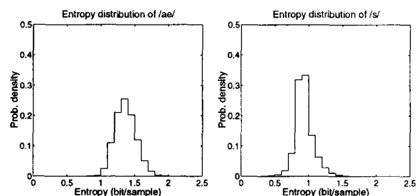
Figure 1: Histograms with the entropy distribution for the Gaussianity based method for /ae/ (left) and /s/ (right).
