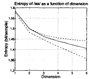
Figure 3: Entropy of quantization indices of unmodified /ae/ (solid), the first-order Markov model (dashed, top curve) and random slope linear phase (dashed-dotted, bottom curve).
