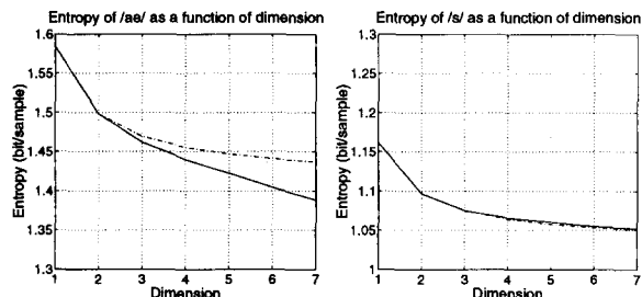
Figure 2: Entropy estimates for the entropy of quantization indices method (solid) for /ae/ (left) and /s/ (right). The dashed-dotted curves are those for a first-order Markov model.
