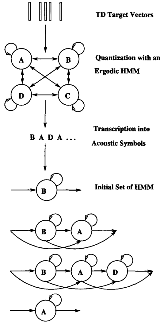
Figure 2. Definition of an initial set of HMM.
