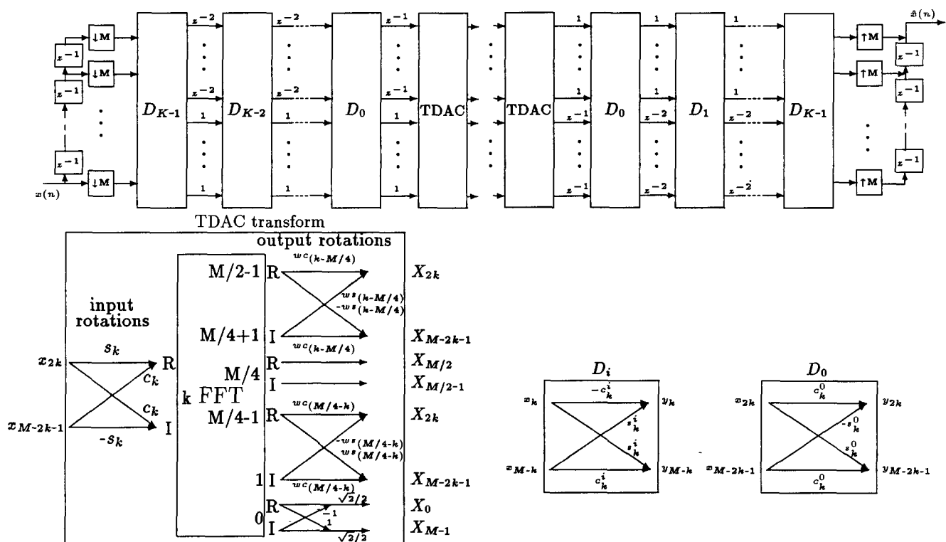
Figure 1: The structure for the fast implementation of the ELT analysis/synthesis filter bank, and the elements of ELT structure: TDAC transform and butterflies. s_k = \sin \theta_k , c_k = \cos \theta_k , \theta_k = (4k + 1)\pi/(4M) , ws_k = \sin(k\pi/M) , wc_k = \cos(k\pi/M) . Note that the butterflies D_i 's and D_0 are different.
