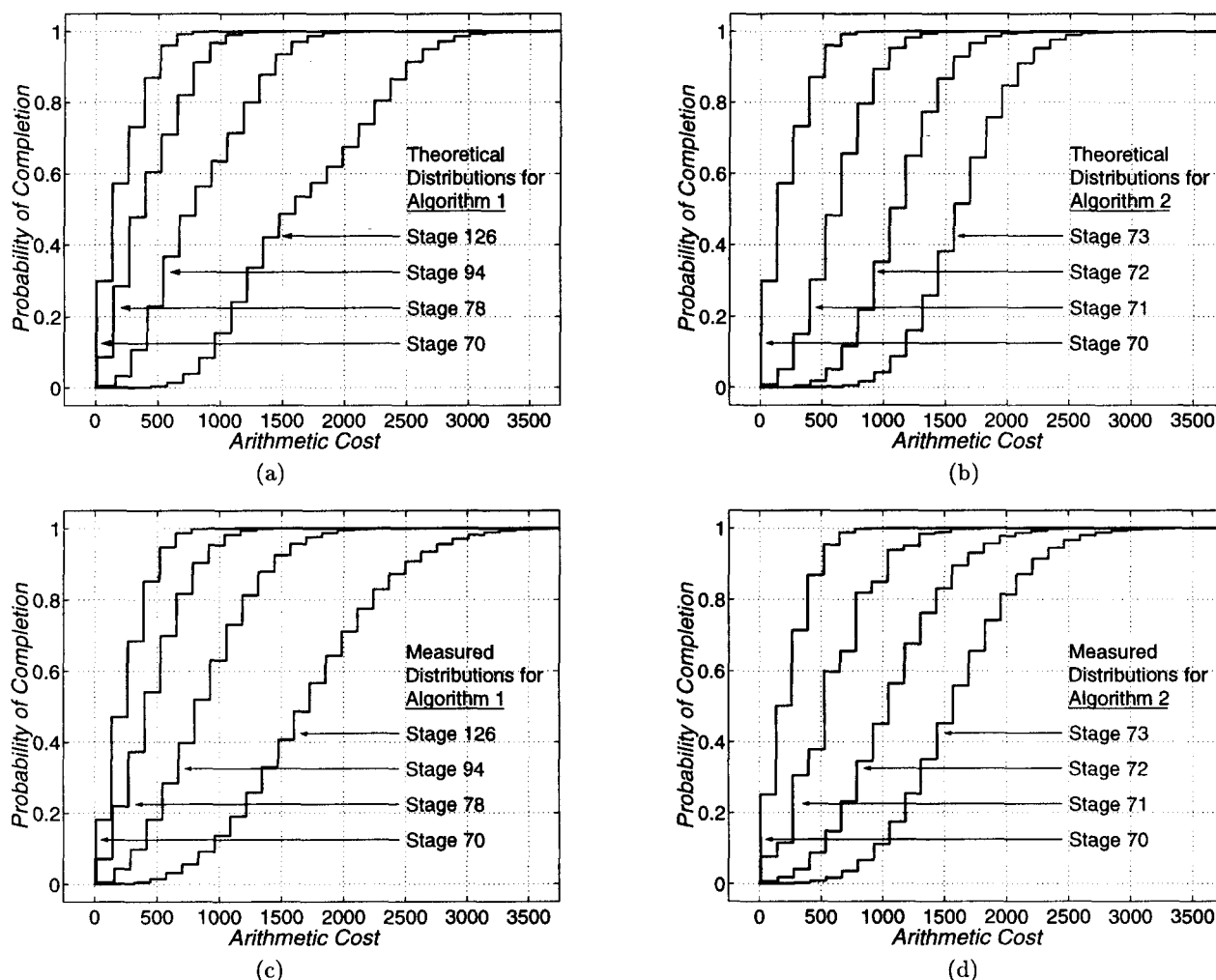
Figure 2: Cumulative probability distributions of the total arithmetic cost associated with completing the DFT-IR algorithm stages given in Table 1. (a) Theoretically predicted distributions for Algorithm 1, Stages 70, 78, 94, 126. (b) Theoretically predicted distributions for Algorithm 2, Stages 70, 71, 72, 73. (c) Experimentally determined distributions for Algorithm 1, Stages 70, 78, 94, 126. (d) Experimentally determined distributions for Algorithm 2, Stages 70, 71, 72, 73.
