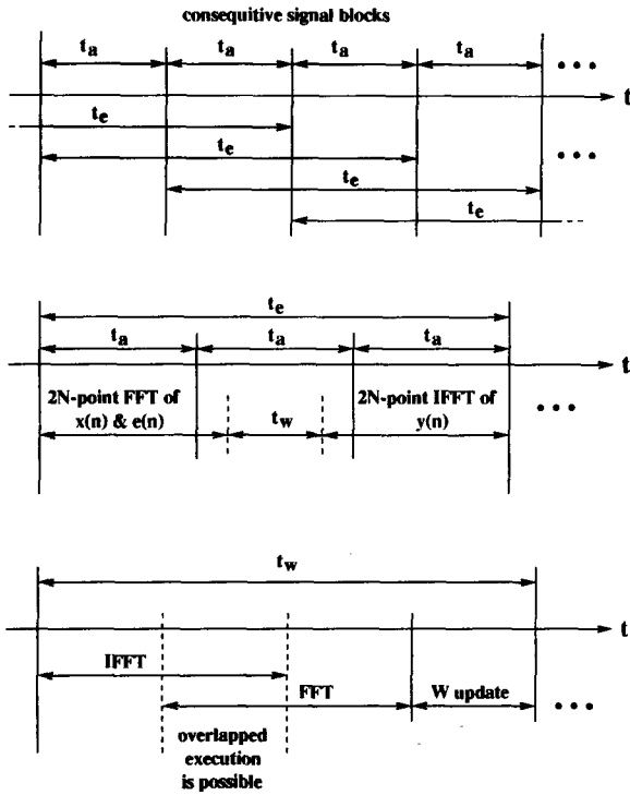
Figure 5. Timing diagrams of a possible frequency-domain adaptive algorithm using sliding transformations. ( t_a denotes the acquisition time of one data block, t_e stands for the execution time of one block adaptation, and t_w for the calculation time of the gradient and the W update). The end-to-end delay is of 2N samples.
