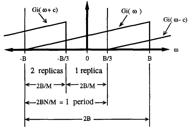
Figure 2. The components of the i -th output channel in the frequency domain when N=2, M=3 .
