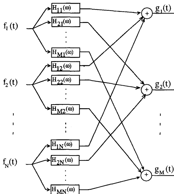
Figure 1. A MIMO LTI system.
