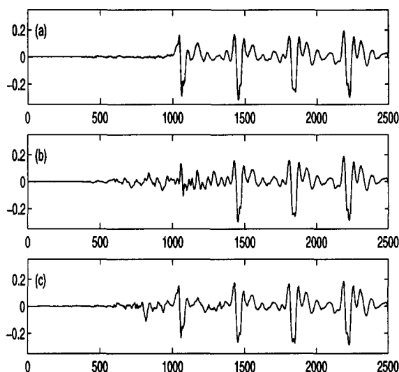
Figure 5. (a) A saxophone attack, (b) its delocalized reconstruction using a fixed frame size (512), and (c) a more accurate reconstruction using dynamic segmentation with the set of sizes {128, 256, 384, 512}; the algorithm chooses sizes 256 and 384 for the first two frames, and 512 for the rest.
