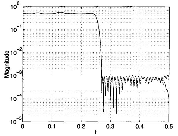
Figure 5: Optimal commutator form filter responses for the projection filter.
