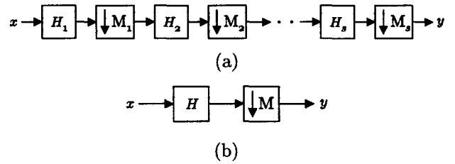
Figure 6: Cascade structure. (a) Multistage form; (b) equivalent single-stage form.
