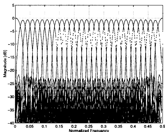
Figure 2. 30-channel paraunitary filter bank with length 60.
