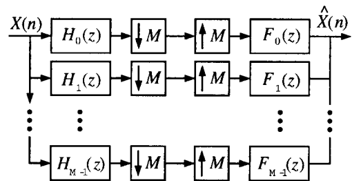
Figure 1. Maximally-decimated M -channel filter bank.
