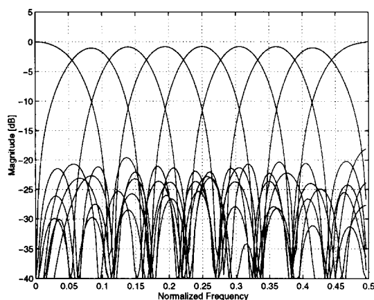
Figure 3. 9-channel paraunitary filter bank with 1-regularity
