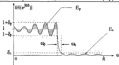
Figure 1: Possible design objectives of filter banks and an illustration of the design objectives of a single low-pass filter. ( [0, \omega_p] is the pass band; [\omega_s, \pi] , the stop band; [\omega_p, \omega_s] , the transition band. )
