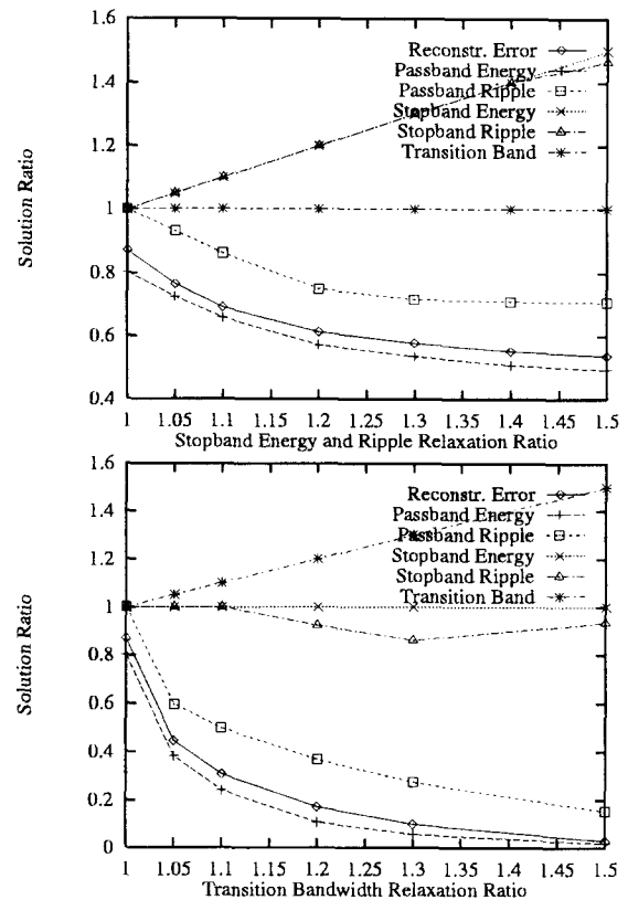
Figure 2: Experimental results in relaxing the constraints with respect to Johnston's designs for 32D QMFs. The x-axis shows the relaxation ratio of stopband energy and ripple (upper), or transition bandwidth (lower) as constraints in NOVEL with respect to Johnston's value. The y-axis shows the ratio of the measure found by NOVEL with respect to Johnston's.
