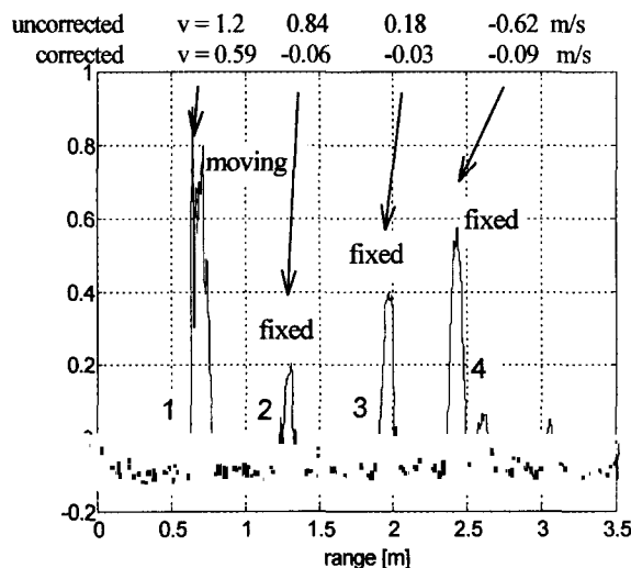
Fig. 5: Echo envelope for 4 targets (1- moving, 2,3,4 -fixed) and their detected velocity before and after applying the correction algorithm
