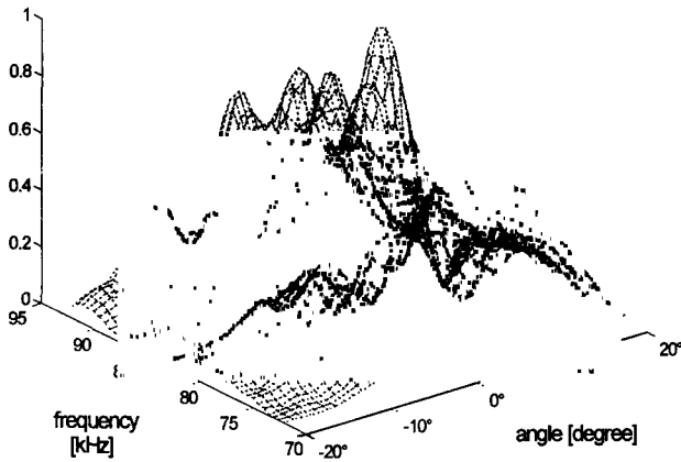
Fig.2: Direction-dependent directivity B(\omega, \psi) pattern of a RU ultrasonic transducer
