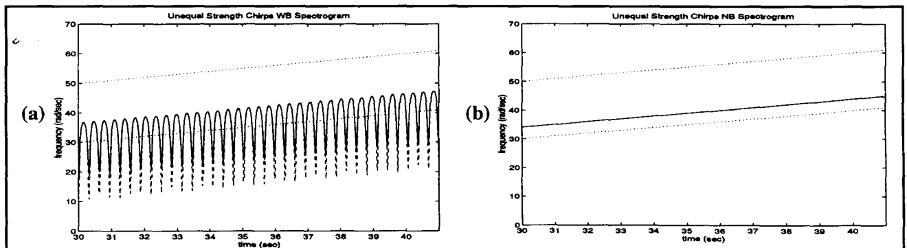
Figure 1: (a) Wideband spectrogram estimate (solid line) of the instantaneous frequency (dashed line) of a signal consisting of the sum of two chirps (dotted lines show individual chirp rates) of unequal strength amplitudes. (b) Narrowband spectrogram estimate (solid line) of the average frequency at each time (dashed line, obscured by estimate) of the same signal. Note that the average frequency at each time, which is a weighted sum of the individual instantaneous frequencies of the two chirps (dotted lines), is generally different from the instantaneous frequency. Interestingly, when the components are of equal strength, these two time-varying frequencies coincide. Similar results hold for the sum of two tones and other signals, as well. See [4], [6], [7], [8] for further details and discussion.
