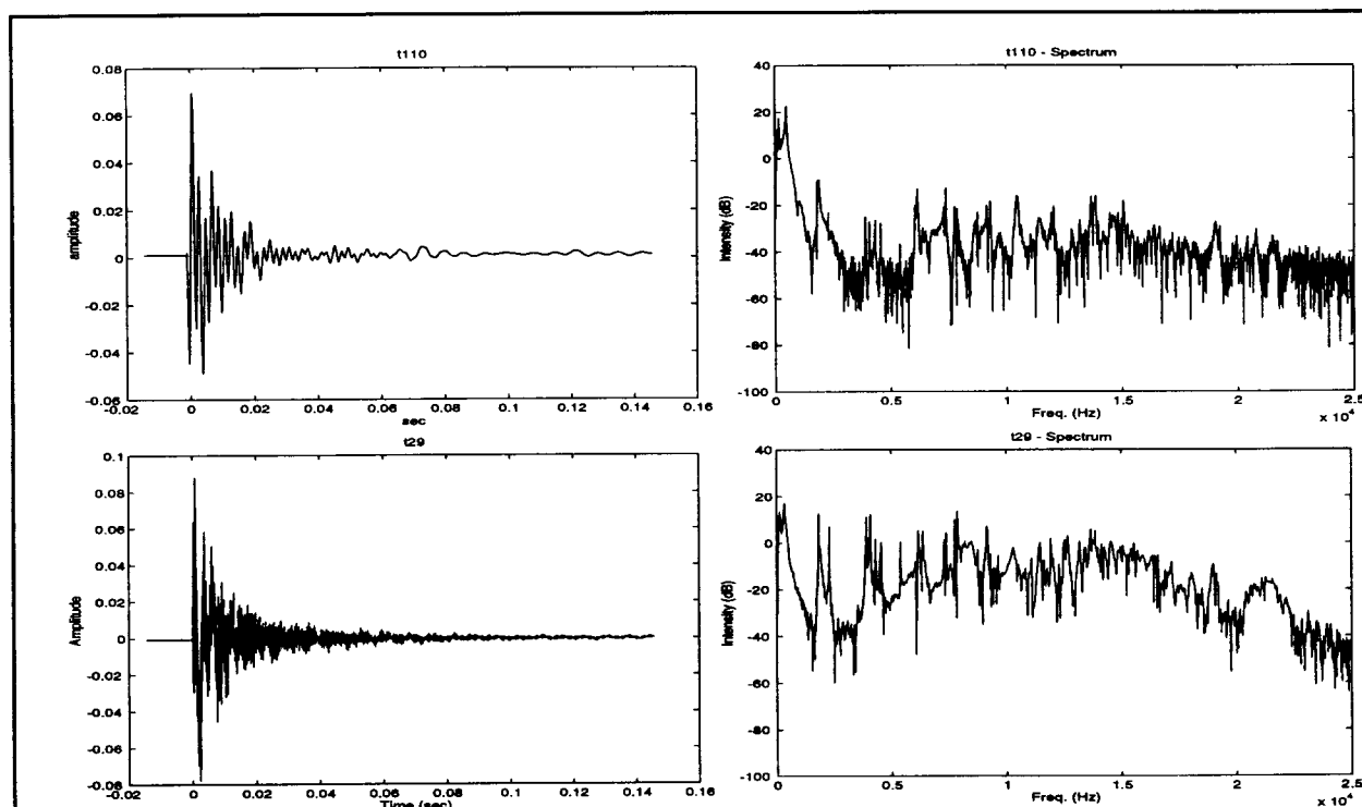
Figure 2: Representative transient time series (left) and spectra (right) from class one (top) and two (bottom).
