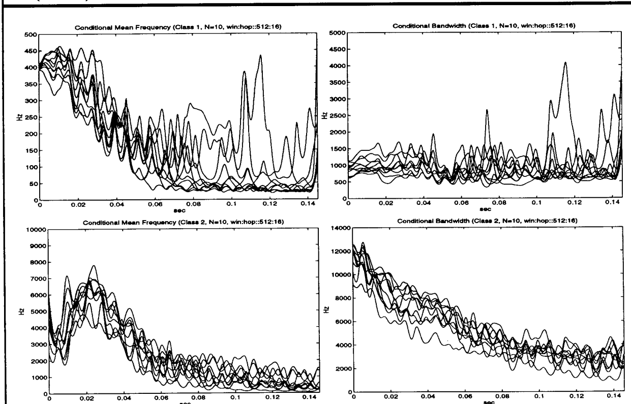
Figure 3: Conditional mean frequencies (left) and conditional bandwidths (right) for each of the ten transients in class one (top) and class two (bottom).
