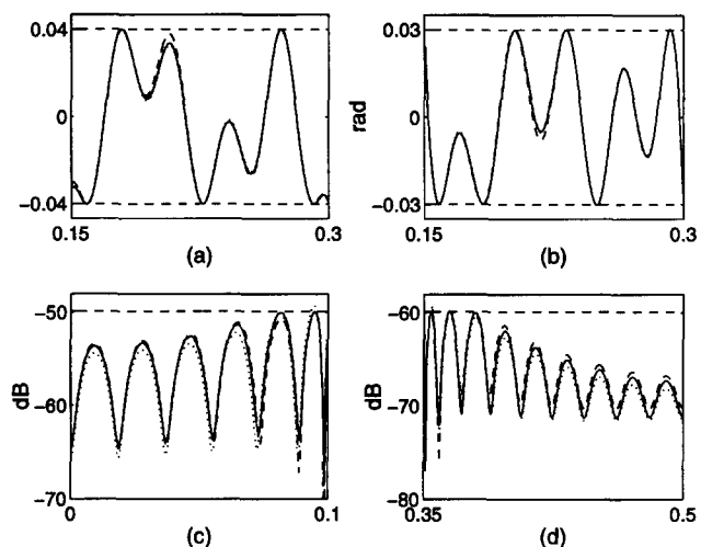
Figure 4: Design example: (a) E_m(2\pi f) in the passband, (b) E_\phi(2\pi f) , (c) |H(e^{j2\pi f})| in stopband 1, (d) |H(e^{j2\pi f})| in stopband 2. Dotted curves: method 1 (alternative 1). Dashed curves: method 1 (alternative 2). Solid curves: method 2.
