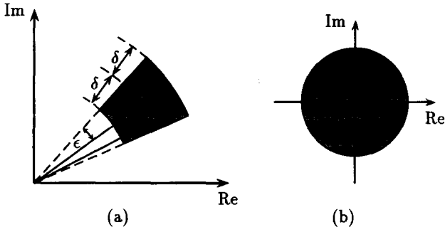
Figure 1: Constraints on magnitude and phase of the frequency response in the complex plane. (a) passbands. (b) stopbands.
