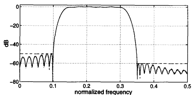
Figure 3: Design example: |H(e^{j2\pi f})| . Dotted curve: method 1 (alternative 1). Dashed curve: method 1 (alternative 2). Solid curve: method 2.
