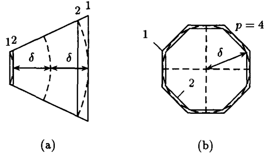
Figure 2: Linear magnitude constraints with (2) and without (1) reduction of the original feasible region. (a) passbands. (b) stopbands (with p = 4 ).
