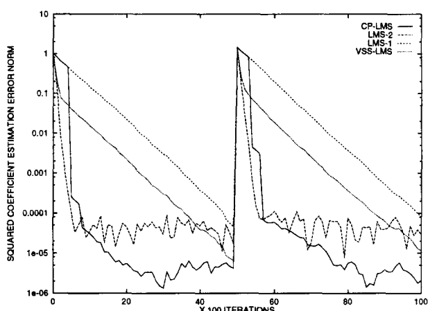
Figure 3. Norm squared estimation error plot
