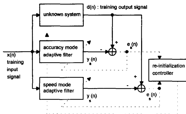
Figure 1. The CP-LMS algorithm block diagram
