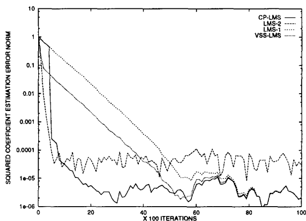
Figure 2. Norm squared estimation error plot
