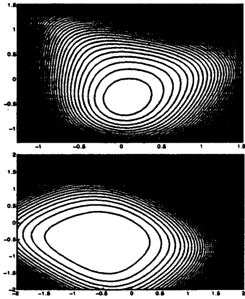
Figure 3. Comparison of the contours of the \|s\|_2^4 - \|s\|_4^4 for channel impulse response [.04 \ .05 \ .07 \ .21 \ .5 \ .72 \ .36 \ .21 \ .03 \ .07] (top) and [.5 \ 1 \ .5] (bottom) and equalizer of length 3 with middle weight fixed at 1.
