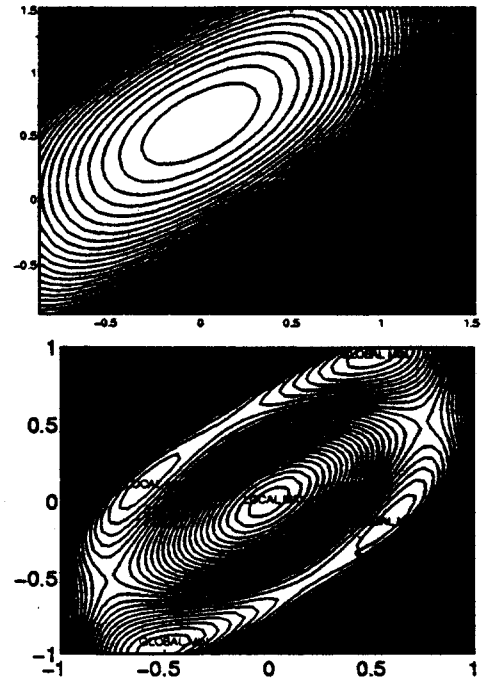
Figure 5. Comparison of the contours of the \|s\|_2^4 - \|s\|_4^4 (top) and Godard-2 (bottom) cost functions. Channel impulse response = [1 \ -0.6 \ .36] .
