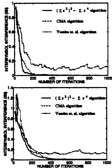
Figure 7. Comparison of the three available algorithms. Input is 4-level QAM, Channel impulse response is [.04 \ .05 \ .07 \ -.21 \ -.5 \ .72 \ .36 \ .21 \ .03 \ .07] , with no added noise (top) and 15db SNR additive white noise (bottom), with 13 adaptive weights.
