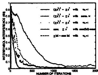
Figure 6. Comparison of five algorithms out of the proposed class of algorithms. Input is 4-level QAM, Channel impulse response is [.04 \ .05 \ .07 \ -.21 \ -.5 \ .72 \ .36 \ .21 \ .03 \ .07] , with 13 adaptive weights and no noise.
