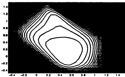
Figure 4. The contour plot of \|s\|_2^4 - \|s\|_3^8 cost function for channel impulse response [1 \ -0.6 \ .36] and equalizer of length 3 with middle weight fixed at 1.
