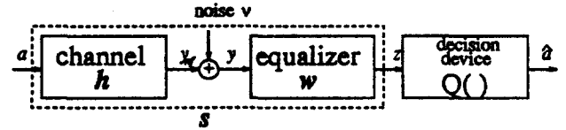
Figure 1. Blind equalization model
