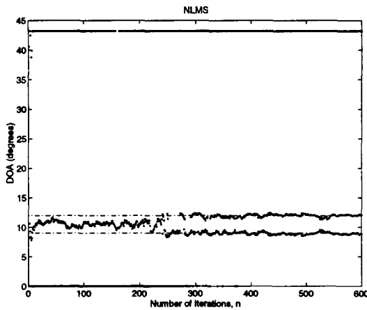
Fig. 1. DOA estimates for two uncorrelated signals at 9° and 12°. NLMS algorithm.
