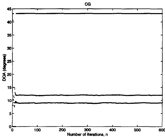
Fig. 2. DOA estimates for two uncorrelated signals at 9° and 12°. CG algorithm.
