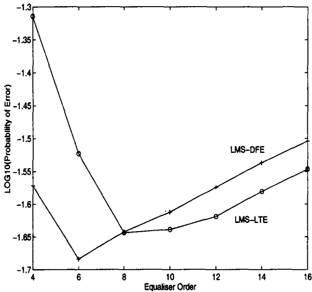
Figure 4: Equaliser order dependency for the LMS LTE and LMS DFE on channel 2 with a fade rate of 2 Hz and a signal-to-noise ratio of 20 dB. The equaliser order corresponds to M - 1 for the LTE and M_f + M_b - 1 for the DFE. For the LTE, the delay is set to (M - 1)/2 . For the DFE, M_b is fixed on M_b = 2 .
