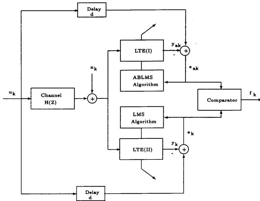
Figure 1: Configuration of the ABLMS LTE in parallel with the LMS LTE. The comparator provides f_k = e_{ak} if (e_{ak})^2 \leq (e_k)^2 and f_k = e_k otherwise. The output of this equaliser is y_{ak} when f_k = e_{ak} , and y_k when f_k = e_k .
