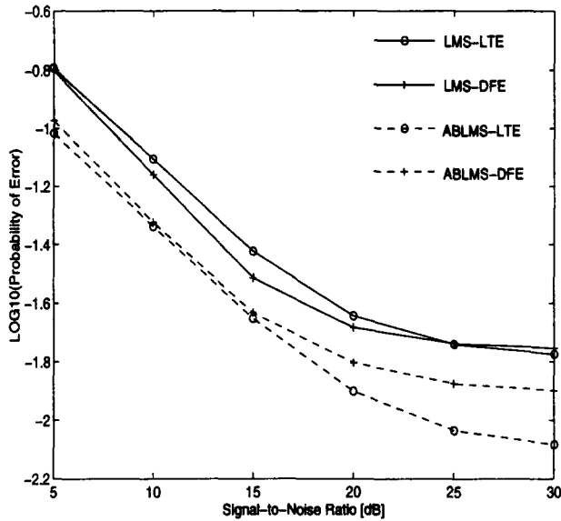
Figure 3: Bit error rate performance against additive noise on channel 2.
