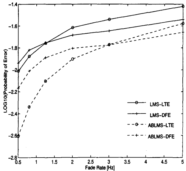
Figure 5: Bit error rate performance against channel fade rates on channel 2.
