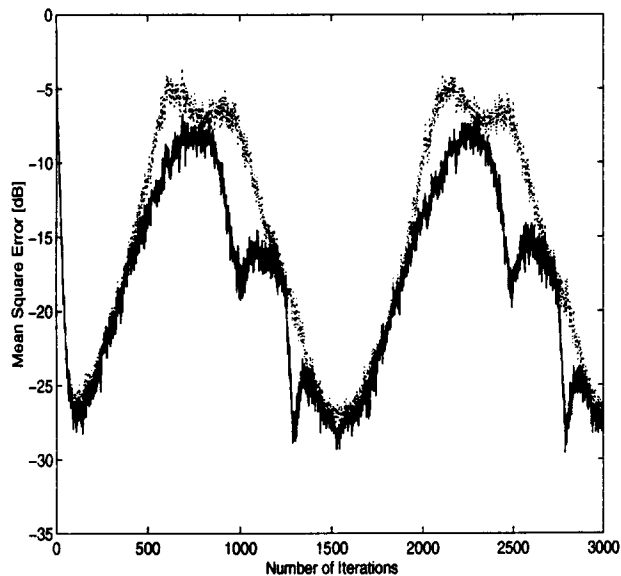
Figure 2: Convergence of the LMS LTE(dotted line) and ABLMS LTE(solid line).
