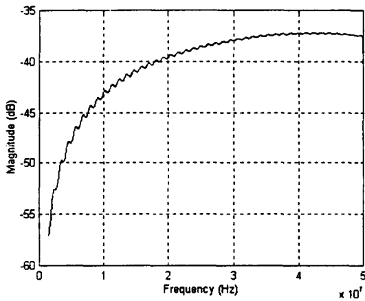
Figure 3. FEXT Loss of A Twisted Pair
