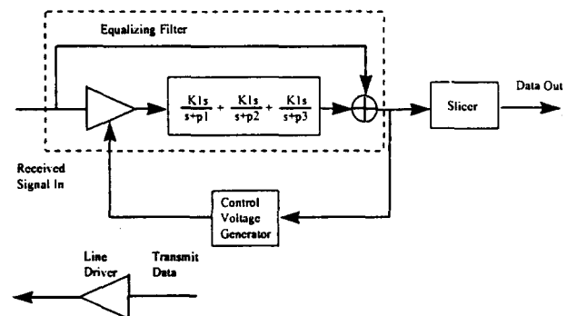
Figure 5. An Analog Adaptive Channel Equalizer
