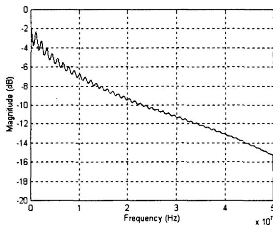
Figure 1. Transfer Function of a Twisted Pair
