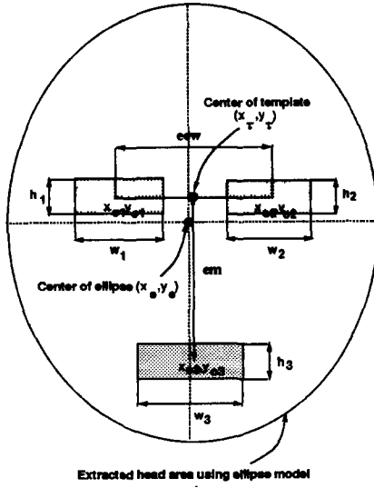
Figure 3. Template used to search eyes and mouth
