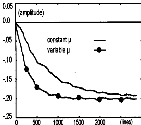
Fig. 2-1 Update curve for the first ghost
