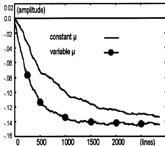
Fig. 2-2 Update curve for the second ghost
