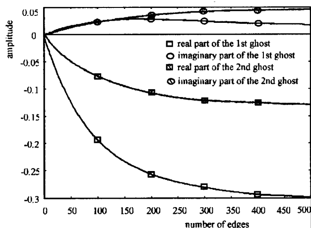
Fig. 4 Update curve only by the sync signals
