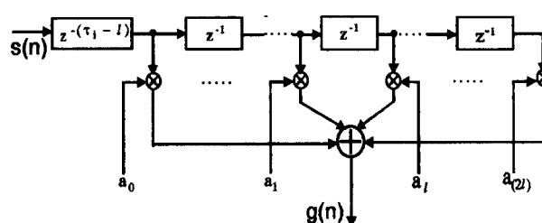
Fig. 3-2 Structure of the i th FIR filter
