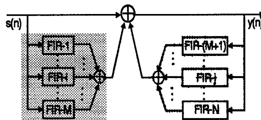
Fig. 3-1 Equalizer structure
