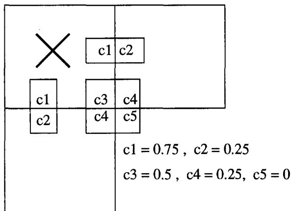
Figure 3. The low-pass filter for the pixels at the block boundary. X is the block being processed
