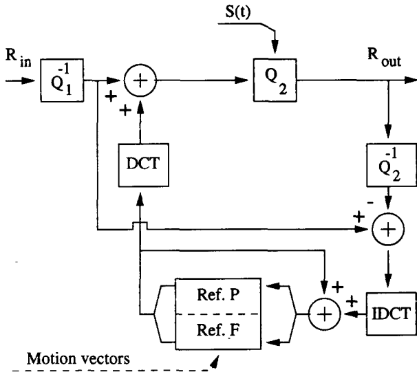
Figure 1. Video transcoder - pixel domain
