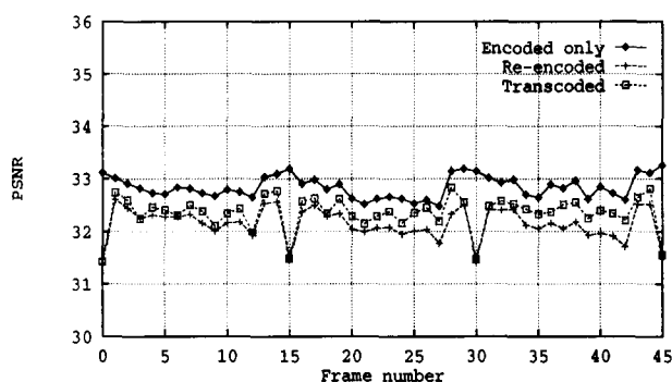
Figure 4. PSNR for VBR transcoding
