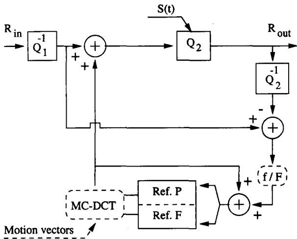
Figure 2. Video transcoder - DCT domain
