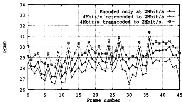
Figure 3. PSNR for CBR transcoding
