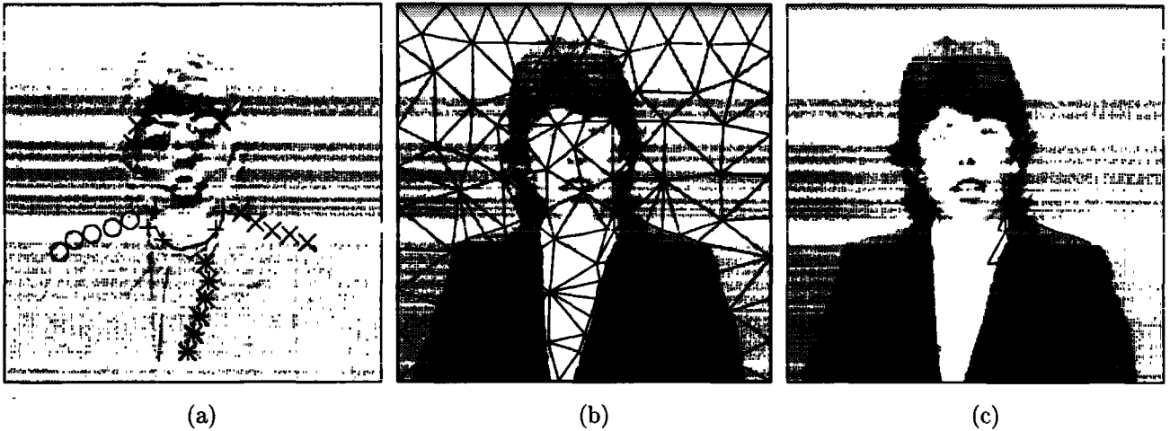
Figure 1: (a) Rip locations for prediction of Frame 5 from 'Claire' (overlaid on top of the frame difference) (b) Final triangulation for prediction of Frame 5 from 'Claire' (c) Translated triangles associated with one rip for prediction of Frame 5 from 'Claire'
