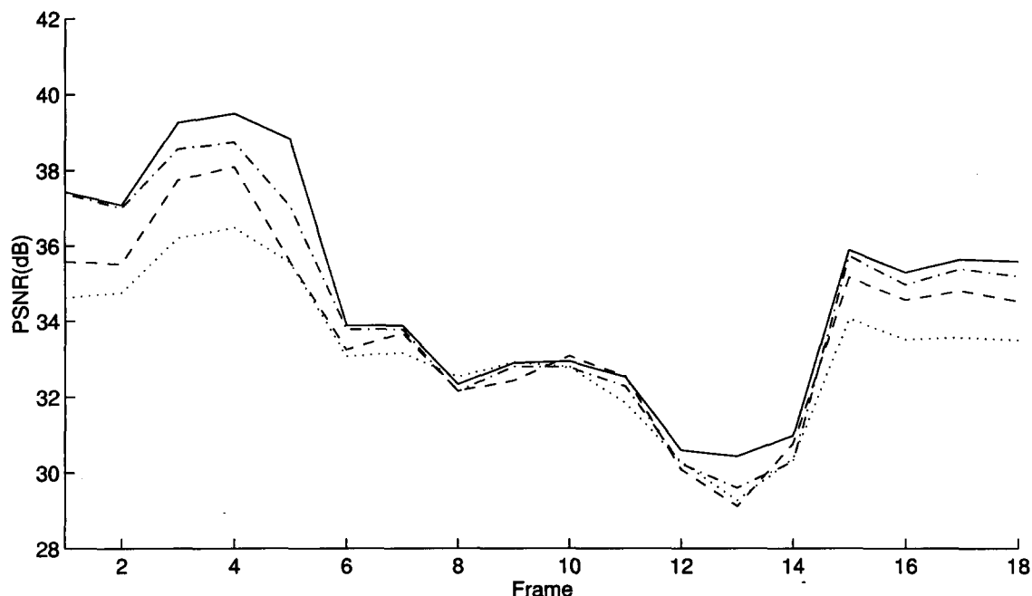
Figure 2: Displaced frame difference errors for the 'Trevor' test sequence
