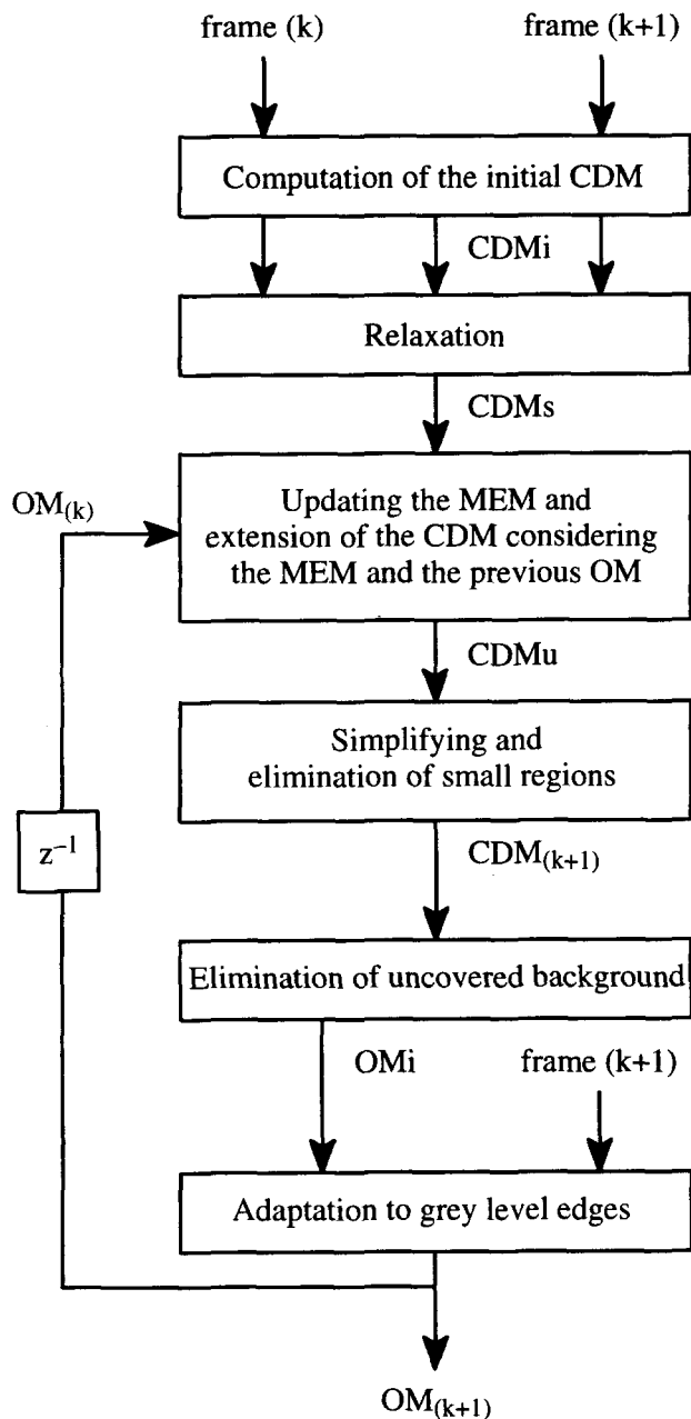
Figure 1: Block diagram of the segmentation algorithm.
