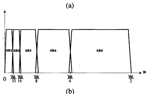
Figure 3. (a) Filter Bank (b) Five unequal-widths subbands in the frequency domain
