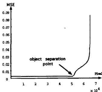
Figure 3. Sorted residual error (MSE) along the epipolar line for all image pixels using the dominant motion parameter set recovered with the LMedS estimator.
