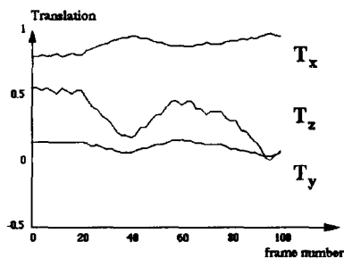
Figure 8. Estimated translation parameters for 100 frames of the Flowergarden sequence.
