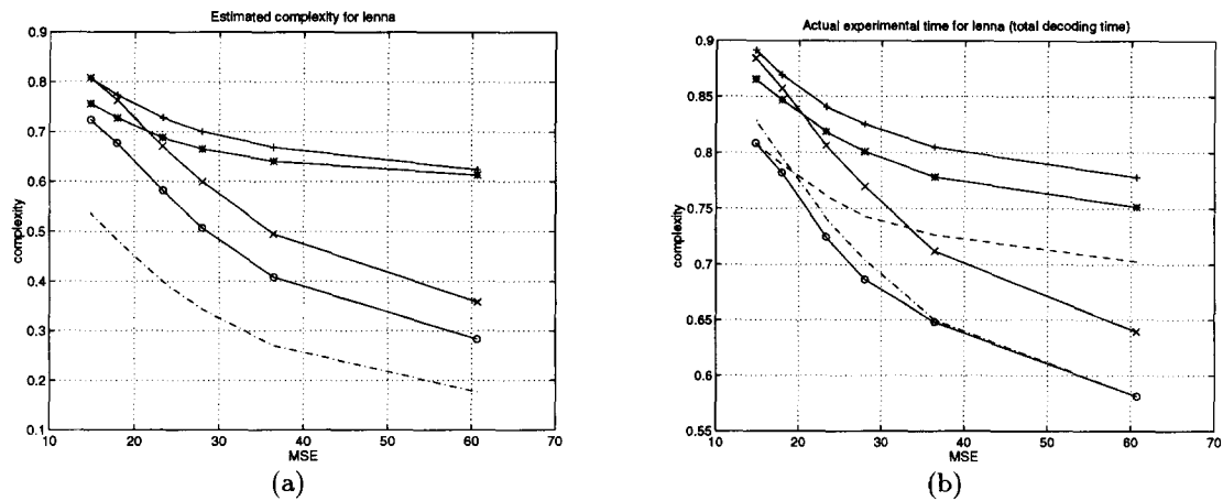
Figure 3. Normalized results for lenna (CW=1): (a) estimated IDCT complexity, (b) experimental decoding complexity. In (a) we compare, CW with all-zero test ('+'), CW with all-zero test for the first 1-D IDCT and ac-zero test for the second 1-D DCT ('x'), FW ('*'), tree-structured classification ('o'), and algorithm with no classification cost ('-'). For (b) we also have results for optimized trees designed with different inputs with MSE=14.8 ('--') and MSE=60.66 ('-').
