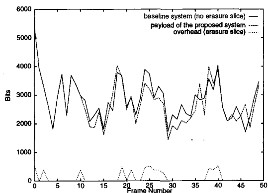
Figure 2: Bit sequences for the baseline and the proposed method
