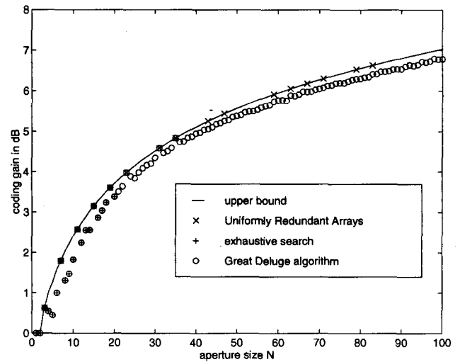
Figure 2. Comparison of one-dimensional apertures designed using the GD algorithm to the upper bound ( \xi \rightarrow \infty ).
