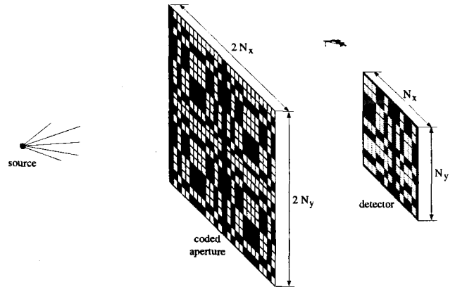
Figure 1. Coded aperture imaging system.
