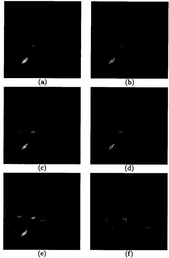
Figure 3: (a) FBP of noiseless projections at correct angles. (b) FBP of noisy projections at correct angles with N_0 = -30\text{dB} . (c) FBP of noiseless projections at MLE angles. (d) FBP of noisy projections at MLE angles. (e) FBP of noiseless projections at initial guess angles (generated by heuristic algorithm). (f) FBP of noiseless projections where angles are assumed correctly ordered and uniformly spaced.
