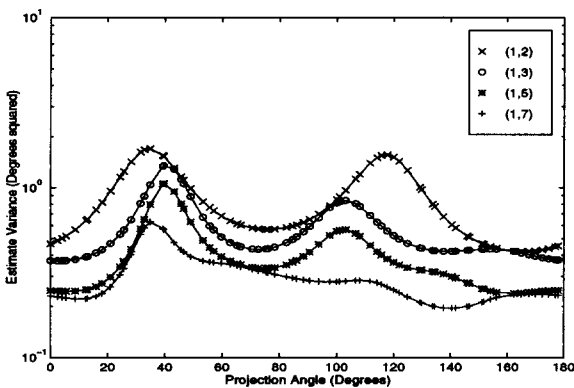
Figure 1: Cramér-Rao bounds for the disk phantom at N_0 = -30\text{dB} for 75 angles (the symbols mark the angles used in the calculations)
