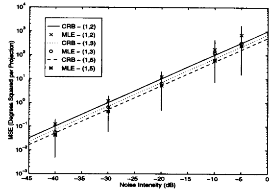
Figure 2: Monte Carlo simulations of the MLE for (1, k) methods.
